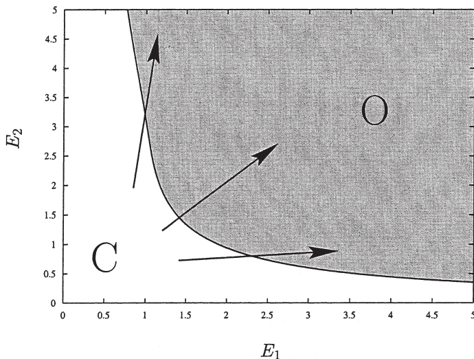
Figure 6. Division of E_2 - E_1 parameter space into convergence ('C') and overshoot and collapse ('O') regions. The arrows indicate possible paths E_2 and E_1 might take as they evolve over time.
