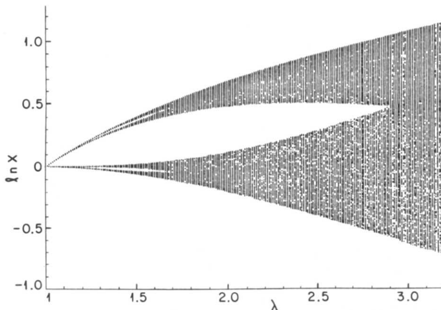
Figure 1 Plot of population values (on a logarithmic scale, \ln(N/N_T) ) generated by iterating equation (2.4) many times, for each of a sequence of \lambda -values. the diagram gives an impression of the probability distribution of population values generated by this purely deterministic difference equation (after May, 1985 28 ).
