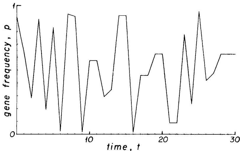
Figure 2 Illustrating the highly chaotic dynamic behaviour of the gene frequency p that can arise once the selective forces exerted by the pathogens are both frequency- and density-dependent. the figure plots successive iterates of p , as generated by the first-order difference equation (4.1) with (4.2) and (4.3) defining the fitness functions. After May and Anderson (1983), 30 where details are given.
