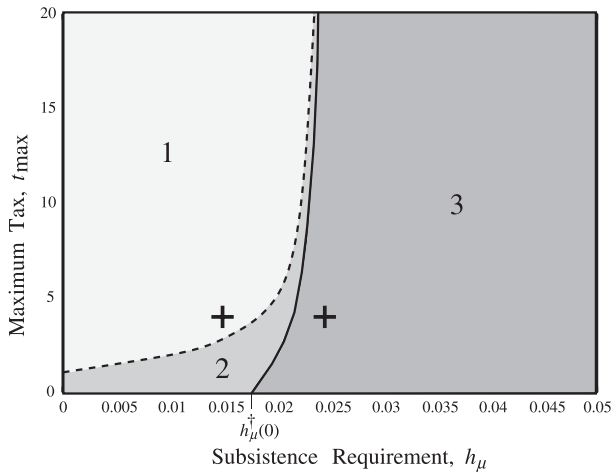
Fig. 5. Regions in h_\mu – t_{\max} parameter space with qualitatively different behavior. In region 1, institutional response will prevent overshoot and collapse. In region 2, the system will experience relatively mild overshoot and collapse and eventually converge to a steady state. In region 3, the system will experience increasingly severe overshoot and collapse as h_\mu increases. The system will either oscillate perpetually or converge to the steady state relatively slowly. The two crosses mark the parameter combinations used for Fig. 4A and B.
