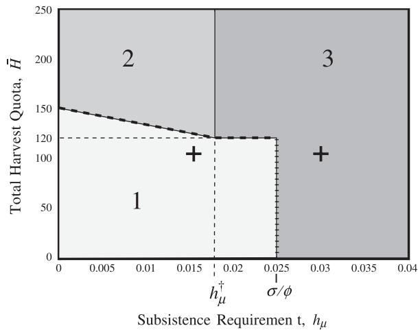
Fig. 6. Regions in h_\mu – \bar{H} parameter space with qualitatively different behavior. In region 1, institutional response will prevent overshoot and collapse. In region 2, the system will experience relatively mild overshoot and collapse and eventually converge to a steady state. In region 3, the system will experience increasingly severe overshoot and collapse as h_\mu increases. The system will either oscillate perpetually or converge to the steady state relatively slowly. The two crosses mark the parameter combinations used for Fig. 7A and B.
