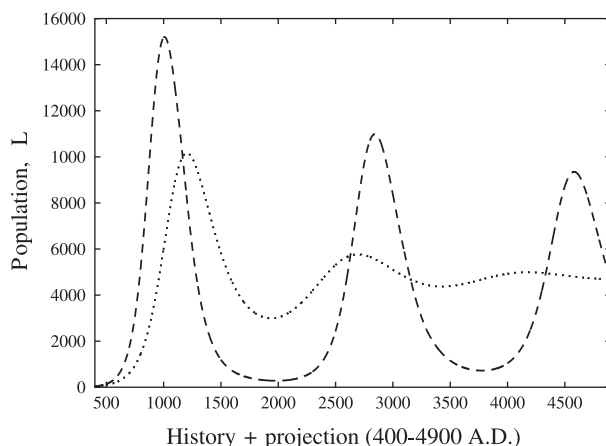
Fig. 2. Population for the BT model (dotted line) and subsistence model (dashed line).
