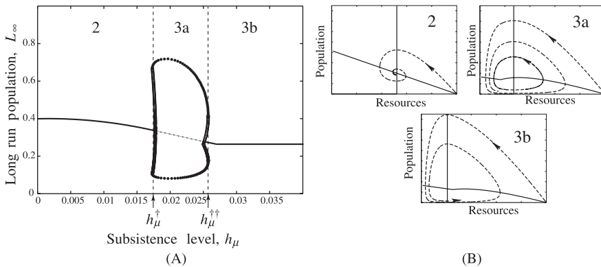
Fig. 3. Figure (A) shows a bifurcation diagram showing fundamental change in long-term behavior as h_\mu is varied. Figure (B) shows the corresponding phase plane diagrams for each of the regions in figure (A). In each figure, the vertical solid line shows the population nullcline (points where \dot{L}=0 , hereafter PN), and the sloping solid line shows the resource nullcline (RN). The dashed line shows a typical trajectory. The subsistence parameter changes the topology of the model in two ways: by shifting the PN to the left and by causing the RN to become curved. The equilibrium point where the PN and RN cross is stable if the slope of the RN is negative as in Region 2. The combination of leftward movement of the PN with the curvature of the RN gives rise to situations in which the slope of the PN is positive at the intersection point as in Region 3a. In this case, the equilibrium point is unstable and the limit cycle emerges. Increasing h_\mu still further shifts the PN further left into the region where the RN becomes linear with a negative slope where again the equilibrium is stable as in Region 3b. However, the topological feature of the curved RN remains, generating severe overshoot and collapse dynamics.
