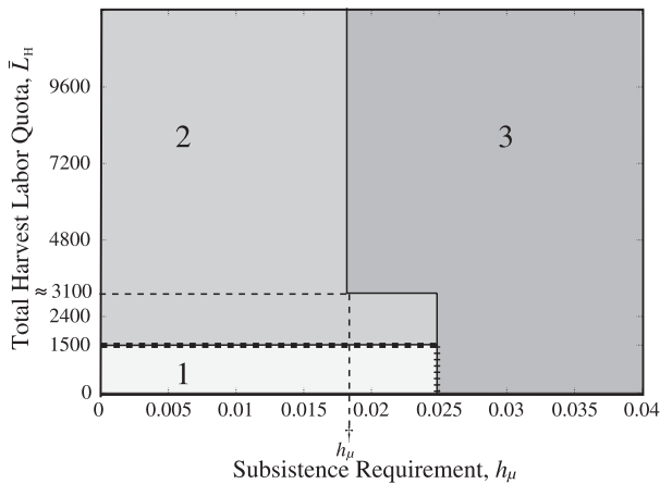
Fig. 8. Regions in h_\mu-\bar{L}_H parameter space with qualitatively different behavior. In region 1, institutional response will prevent overshoot and collapse. In region 2, the system will experience relatively mild overshoot and collapse and eventually converge to a steady state. In region 3, the system will experience increasingly severe overshoot and collapse as h_\mu increases. The system will either oscillate perpetually or converge to the steady state relatively slowly.
