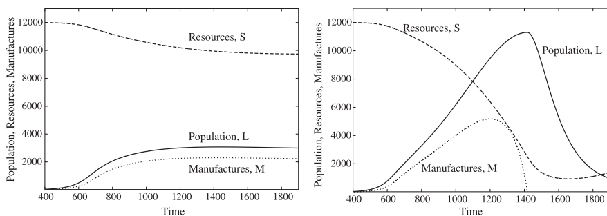
Fig. 4. Figure (A) shows the population (solid line), resource stock (dashed line) and manufacturing output (dotted line) for the subsistence model with the parameter set in column three of Table 1, and a maximum tax strength t_{\max} = 5 . Figure (B) shows the same variables for the same model, but with subsistence h_{\mu} = 0.025 instead of 0.015.
