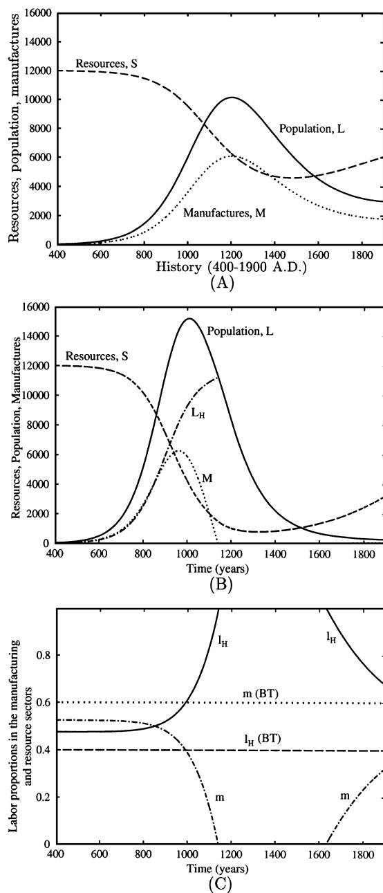
Fig. 1. Figure (A) shows the population (solid line), resource stock (dashed line) and manufacturing output (dotted line) on Easter Island for BT's model (where the subsistence requirement h_\mu = 0 ). Figure (B) shows the same, with the addition of total harvesting labor L_H (dot-dash line), for h_\mu = 0.015 . Figure (C) shows the labor allocations over time as a proportion of the total labor force for the BT model and for h_\mu = 0.015 , as labelled.
