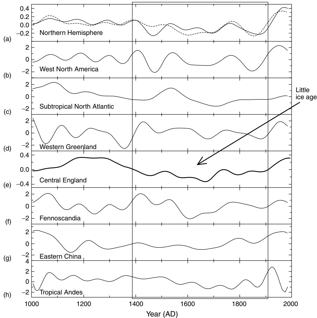
Figure 2 Estimated relative temperature variations during the past millennium for different regions. The records have been smoothed to emphasize century and longer-term variations. (a) Northern Hemisphere mean temperatures as estimated for the annual mean over the entire hemisphere (solid – Mann et al. , 1998, 1999) and over the extratropical region during the warm season (dashed – Jones et al. , 1998) based on global databases of proxy climate indicators, (b) tree ring data from western North America, (c) sediment record from the Sargasso Sea of the tropical North Atlantic, (d) ice cores from western Greenland, (e) a combination of thermometer, historical and proxy data records from central England, (f) tree ring data from Fennoscandia, (g) phenological evidence from eastern China and (h) ice core data from the tropical Andes of South America. Temperature scale is in °C for (a) and (e), and indicates relative temperature variations otherwise. Panel (e), which best defines the European Little Ice Age, is highlighted, with the large rectangle (extending from about AD 1400 to 1900) indicating more broadly the consensus among regions of the coldest period
